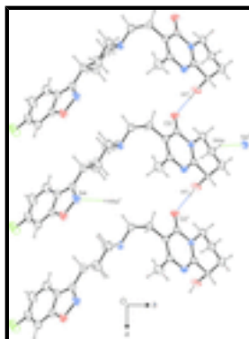
Fig. 2. Selected intermolecular contacts, viewed along [0 0 -1]. For clarity, only the main components of the disordered parts of the molecule are depicted. Blue dashed lines indicate classical hydrogen bonds of the O—H \cdots O type, green dashed lines indicate C—H \cdots N contacts. Symmetry operators: i x - 1, y, z ; ii x - 1, -y + 1/2, z - 1/2 ; iii x + 1, -y + 1/2, z + 1/2 ; iv x + 1, y, z .
