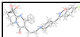
Fig. 1. The molecular structure of the title compound, with atom labels and anisotropic displacement ellipsoids (drawn at 50% probability level).
