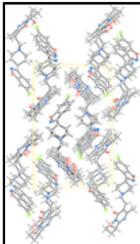
Fig. 3. Molecular packing of the title compound, viewed along [-1\ 0\ 0] (anisotropic displacement ellipsoids drawn at 50% probability level). For clarity, only the main components of the disordered part of the molecule are depicted.
